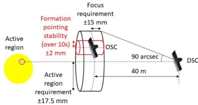
Figure 3. VISORS GNC Science Observation Requirements. 2
