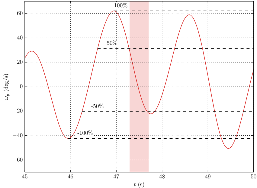
Figure 12. The pitch rate condition is satisfied when the pitch rate percentage is decreasing and between -50% and 50%.
