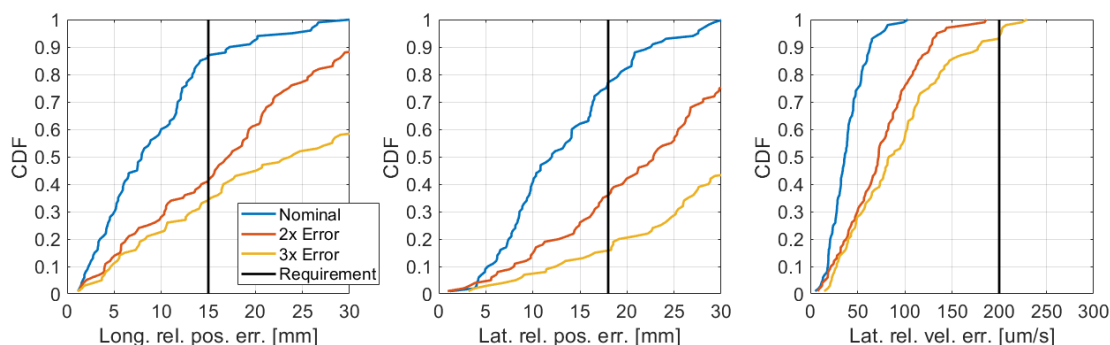
Fig. 19 Comparison of error metric CDFs for nominal, double, and triple relative navigation errors.
