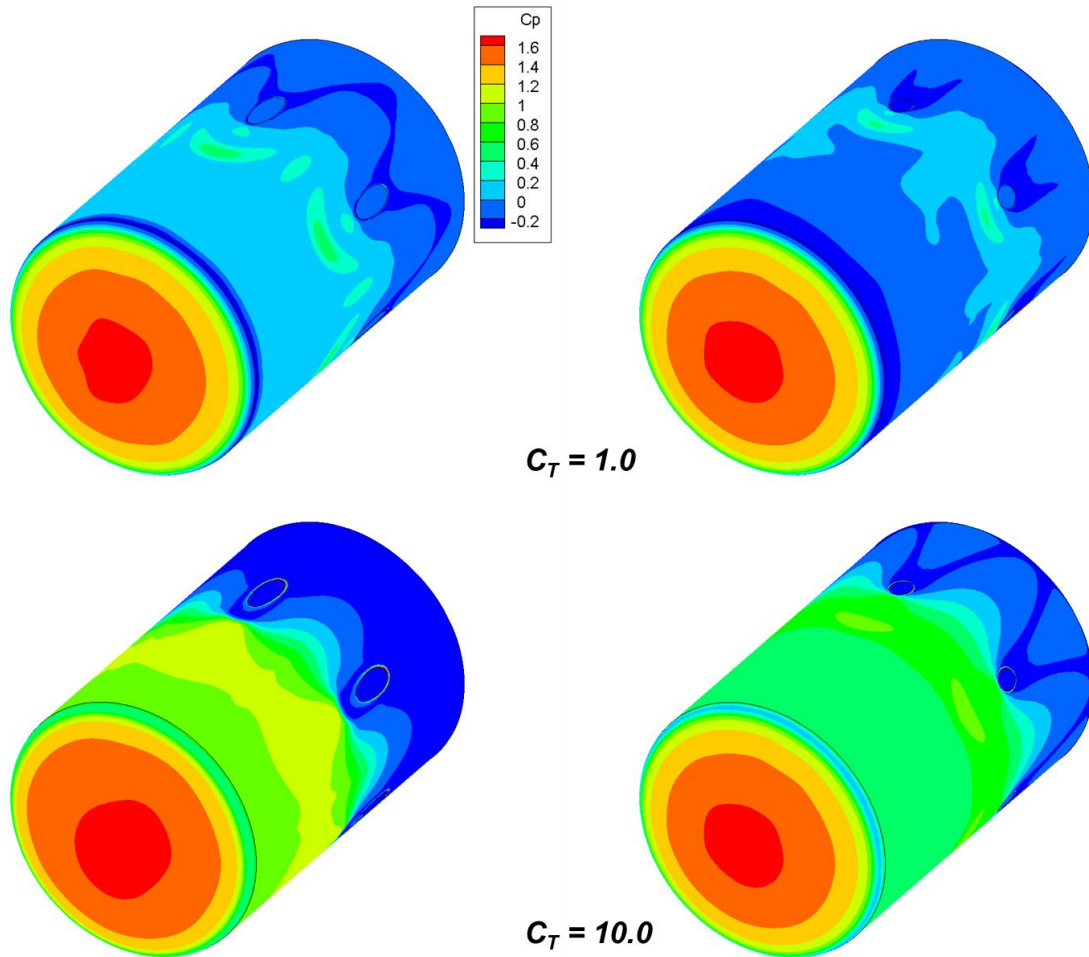
Figure 143: Comparison of pressure distributions between 30° nozzle canting (left) and 60° nozzle canting (right) for six nozzle aftbody configurations
