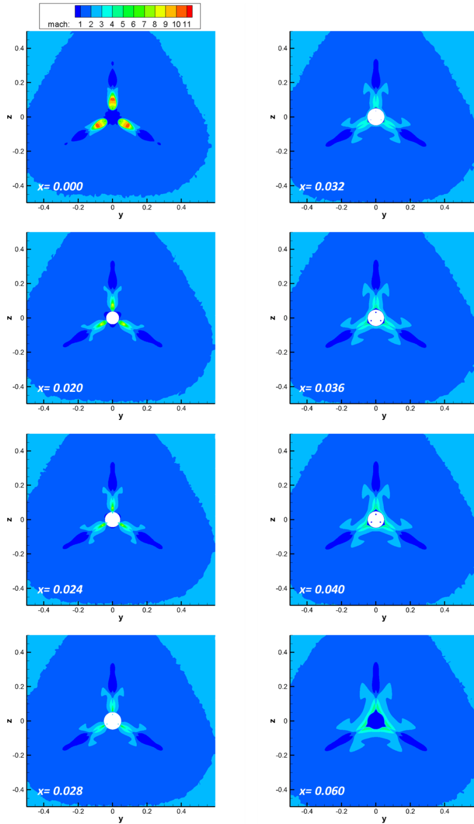
Figure 97: Plume and separated flow interaction for C_T = 10 on the 30^\circ nozzle canting geometry
