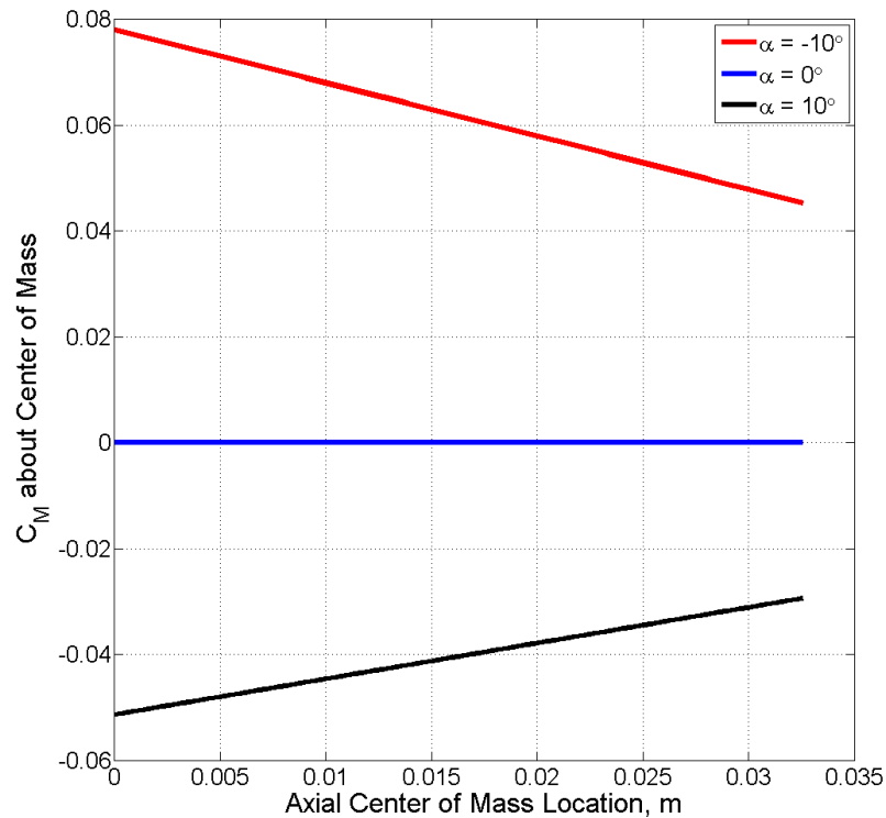
Figure 99: Variation in pitching moment coefficient with center of mass location and angle of attack for C_T = 1 on the 30° nozzle canting geometry
