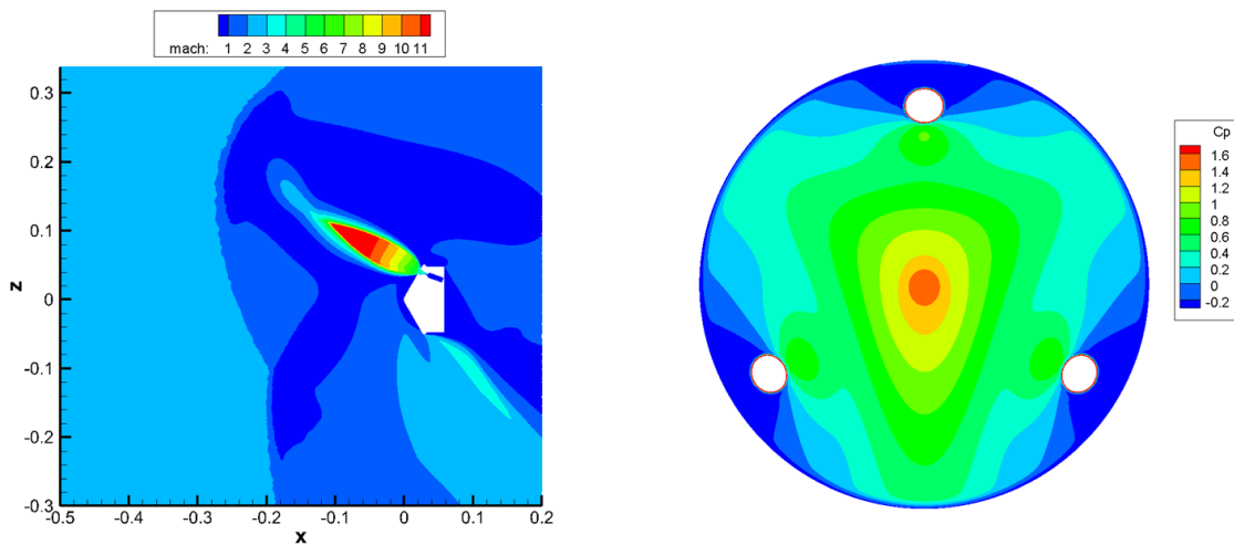
Figure 92: Mach contours and C_p distribution for C_T = 10 , \alpha = -20^\circ with 20^\circ nozzle canting
