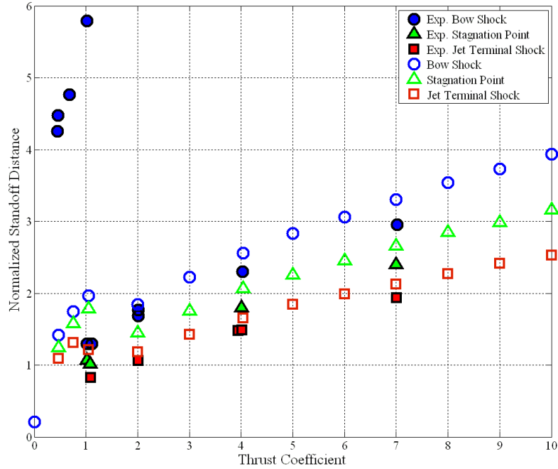
Figure 31: Axial flow structure locations for varying C_T for the single nozzle configuration
