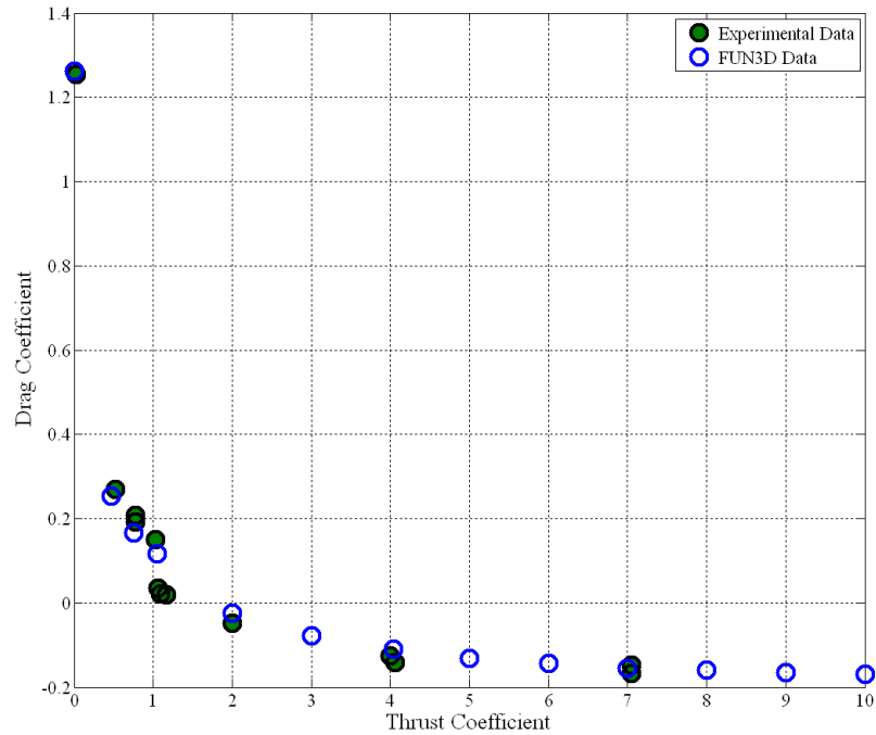
Figure 34: Integrated forebody C_D variation with C_T for the single nozzle configuration
